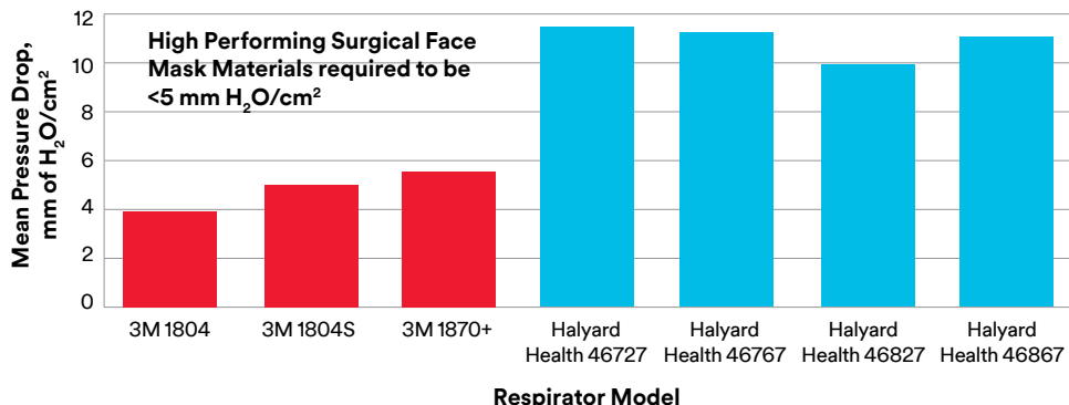
Surgical N95 Respirator Differential Pressure (Delta-P) Study
